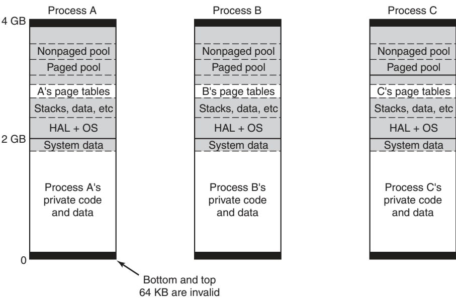
Figure 11-28. Virtual address space layout for three user processes on the x86. The white areas are private per process. The shaded areas are shared among all processes.
